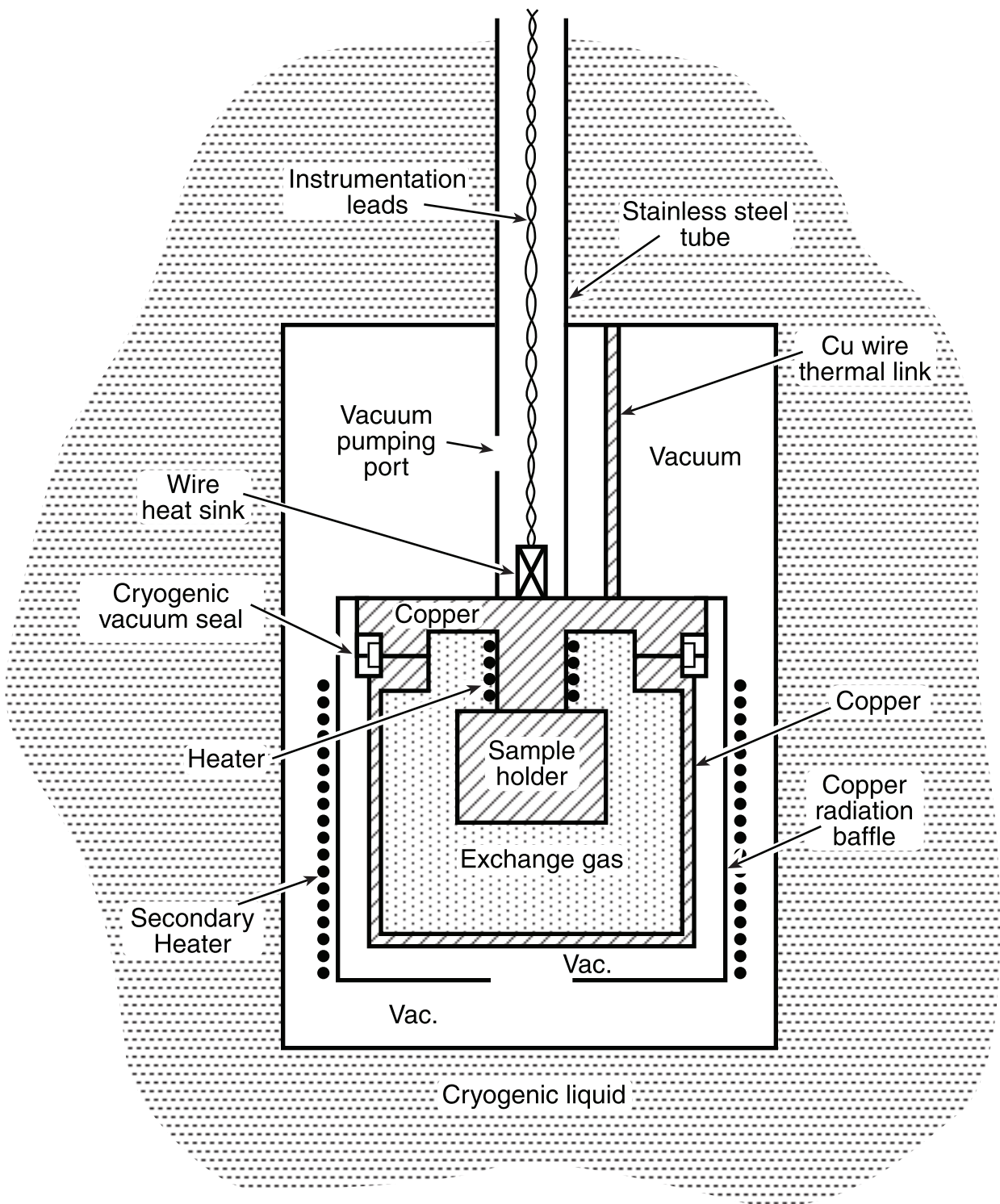
FIG. 2.13. Schematic diagram of vacuum-jacketed variable-temperature sample chamber.
