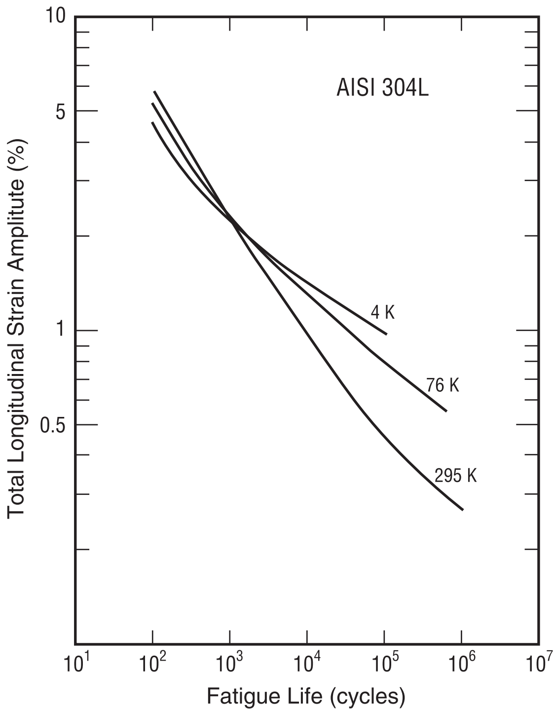
FIG. 6.22 Strain-cycling fatigue curves for AISI type 304L austenitic stainless steel at 295 K, 76 K, and 4 K (from Nachtigall 1975).
